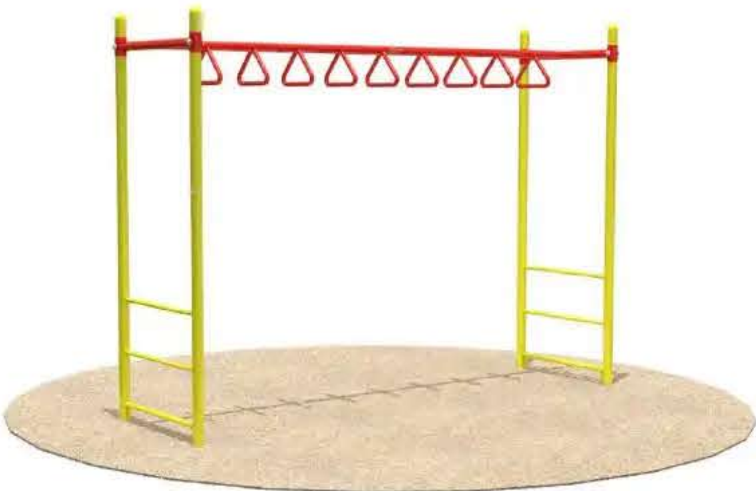
Monkey Bar Climber TPS-01-CL Dimension - 3.1 x 0.9 x 2.4 m. (10 x 3 x 8 ft.)
