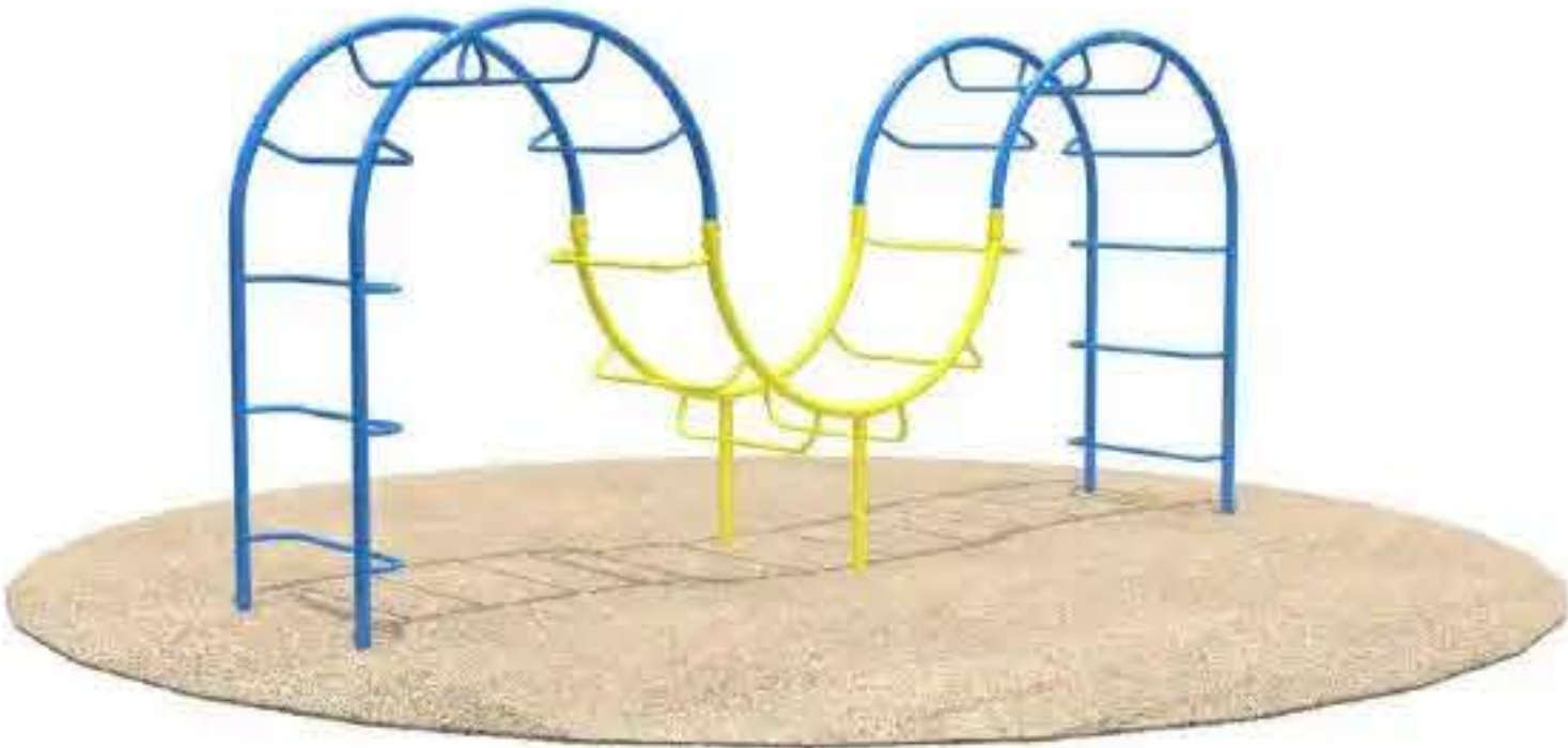
Snake Climber TPS-05-CL Dimension - 4.3 x 0.9 x 2.2 m. (14 x 3 x 7.4 ft.)
